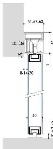
Fixation murale
