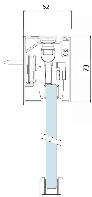
Fixation murale
